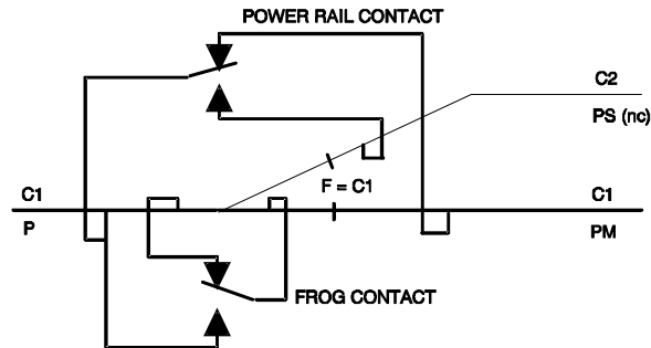
Figure 7-6 Power Routing With Straight Stock Rail Common
