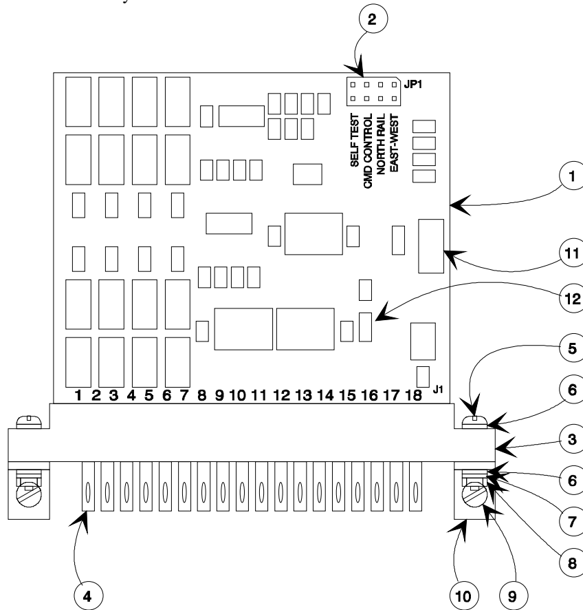
Figure 8-3 BD8 Board Assembly Diagram
