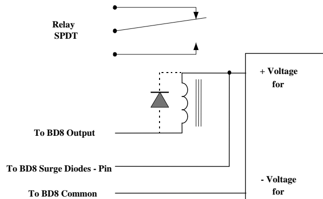
Figure 8-15 Connecting Inductive Loads
