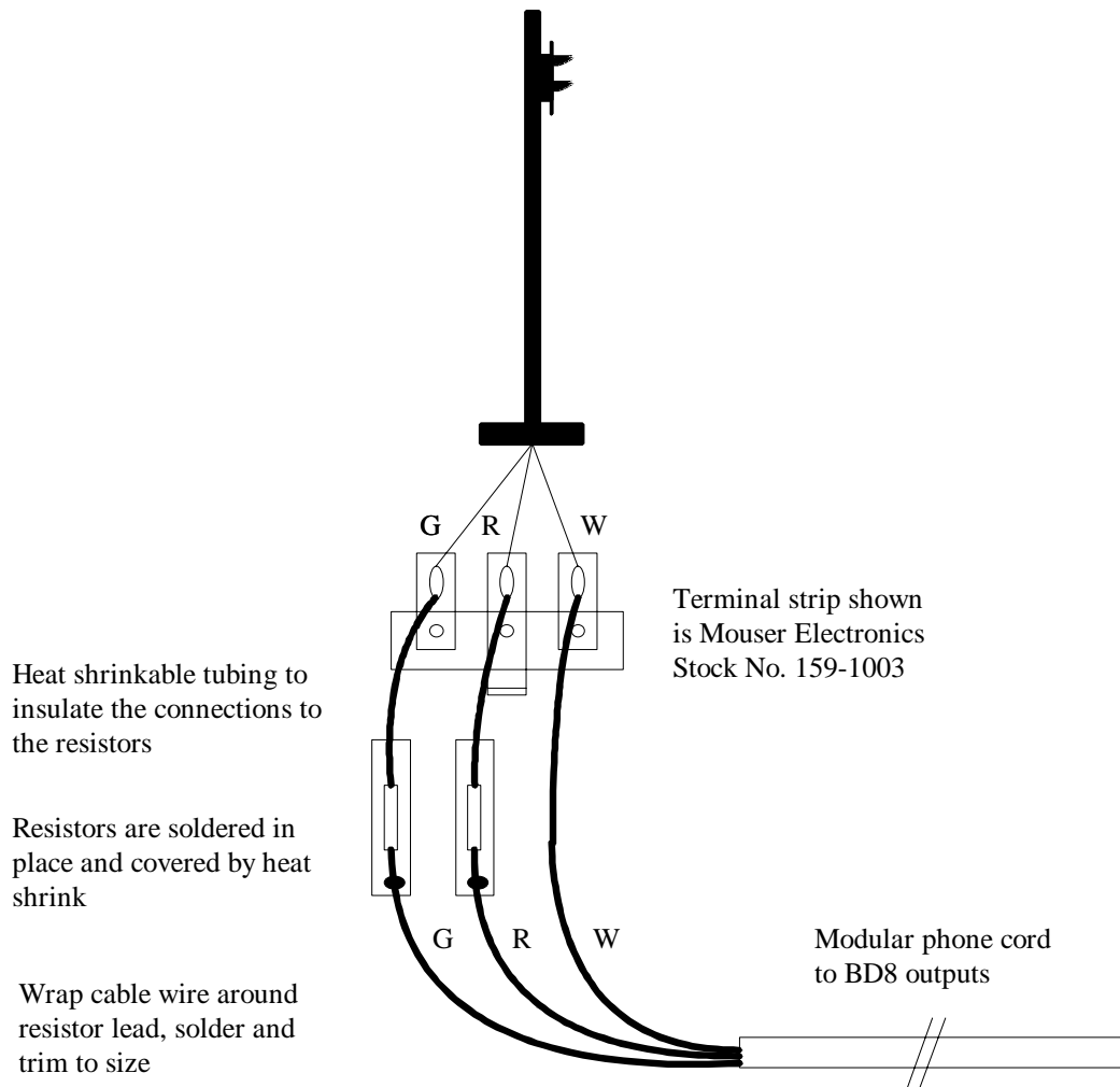
Figure 8-14 LED Resistor Installation Method
