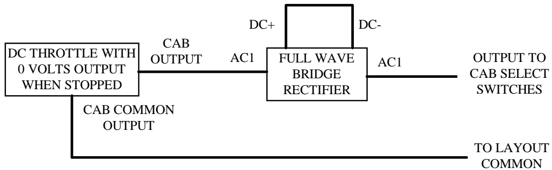
Figure 8-17 Zero Output Throttle Modification
