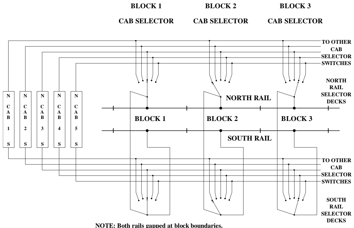
Figure 4-1 Two Rail Switched Cab Circuits
