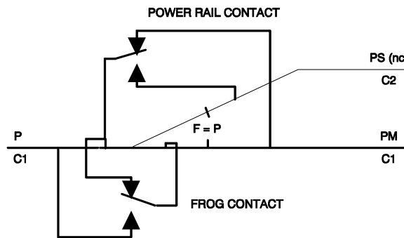
Figure 7-4 Power Rail Routing to Main Line
