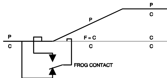
Figure 7-2 Power Routing Switch Set For Siding
