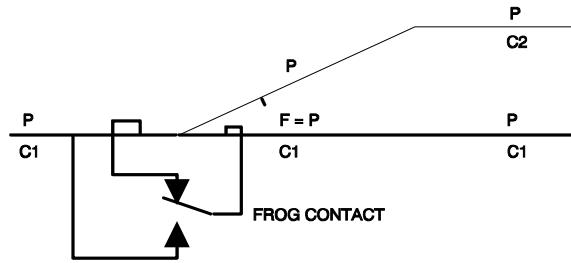
Figure 7-3 Power Routing and Separate Siding Detection
