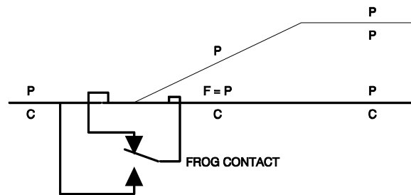
Figure 7-1 Power Routing Switch Set For Main Line
