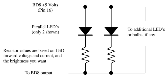
Figure 8-13 Driving Multiple LED's From a Single Output
