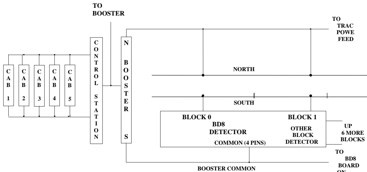
Figure 8-1 DC Control with BD8 Detector Board
