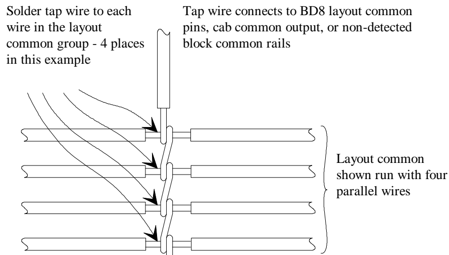
Figure 6-1 Tap Wire Connected to Layout Common
