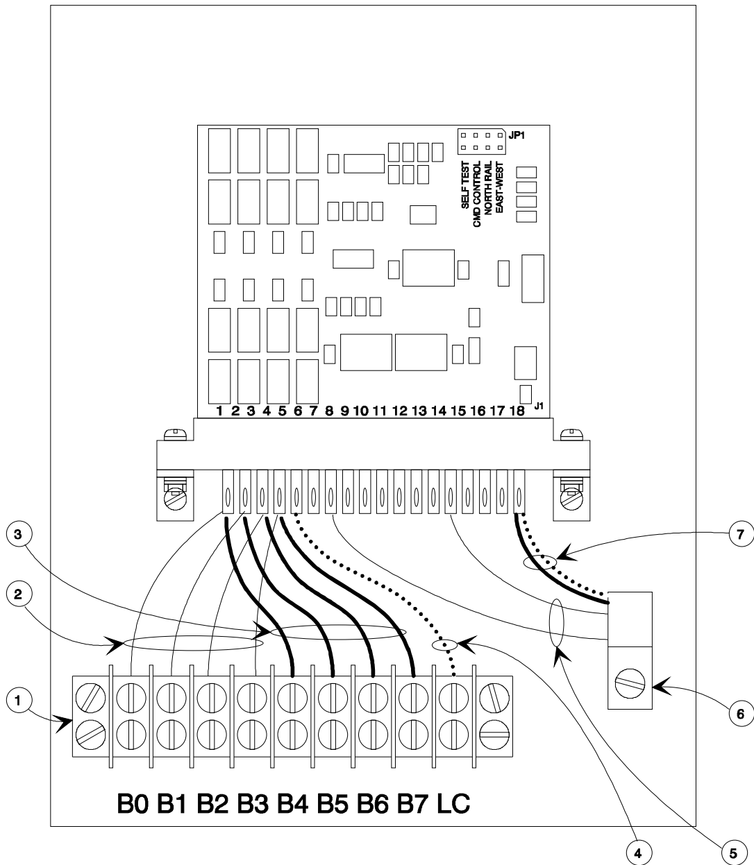
Figure 8-4 BD8 and Panel Layout Ready
