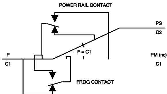
Figure 7-5 Power Rail Routine to Siding
